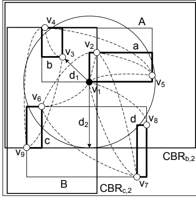
Fig. 6 An example of processing a GSGQ_{rkNN} Q_{gs} = (v_1, rkNN, 2) .
