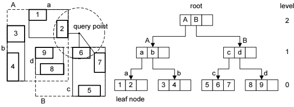
Fig. 2 An example of R-tree.
