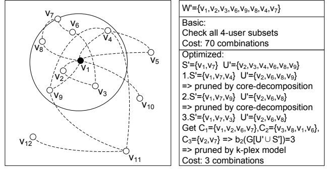
Fig. 7 Exemplary procedures of the original and optimized function FindExactkNN when W' = \{v_1, v_2, v_3, v_6, v_9, v_8, v_4, v_7\} for GSGQ_{kNN} Q_{gs} = (v_1, 3NN, 2) . The entries are omitted here because they are not related to function FindExactkNN .
