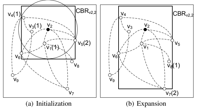
Fig. 4 An exemplary procedure of computing CBR_{v2,2} in an LBSN. The number after a user v_i denotes the core number of v_2 in the subgraph determined by v_i . For a), the subgraph is formed by the users inside \odot_{v2,v_i} ; for b), the subgraph is formed by the users inside CBR_{v2,2} when moving its bottom edge outward to go through v_i .
