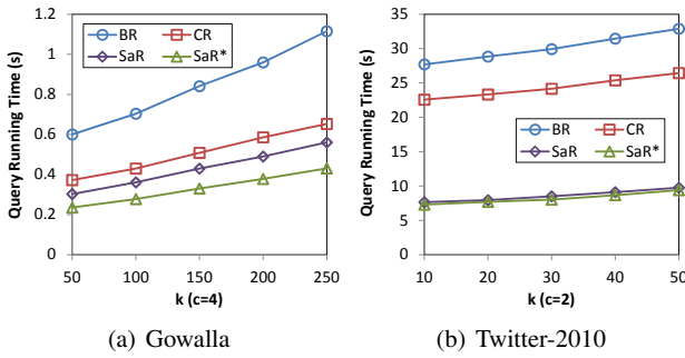
Fig. 16 Query running time of the methods for GSGQ_{rkNN} queries with different k settings.
