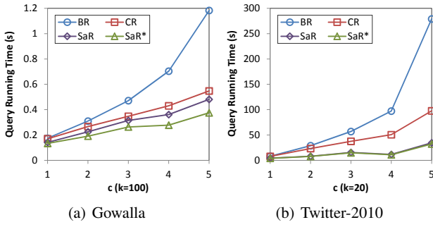
Fig. 15 Query running time of the methods for GSGQ_{rkNN} queries with different c settings.
