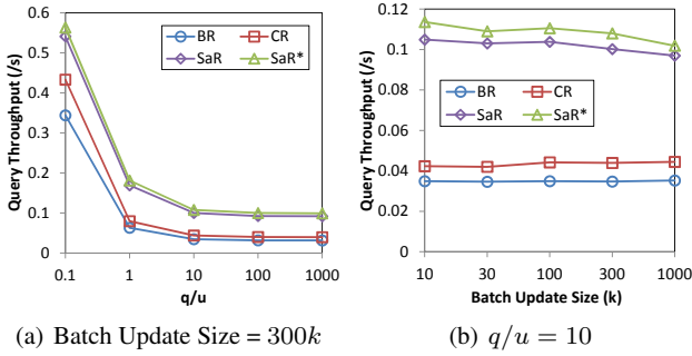
Fig. 20 The query throughput of the methods on Twitter-2010.
