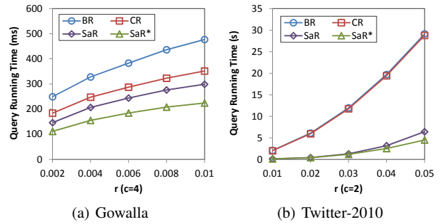
Fig. 14 Query running time of the methods for GSGQ_{range} queries with different r settings.
