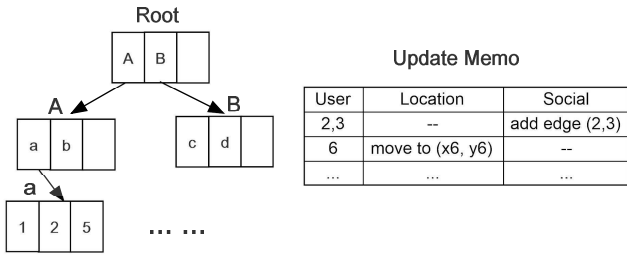
Fig. 8 Lazy Update and Update Memo
