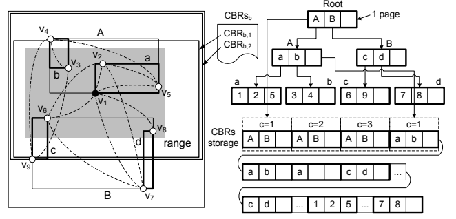
Fig. 5 SaR-tree. CBRs_e denotes the set of CBRs for an entry e .
