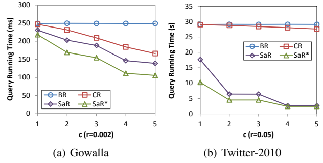
Fig. 13 Query running time of the methods for GSGQ_{range} queries with different c settings.
