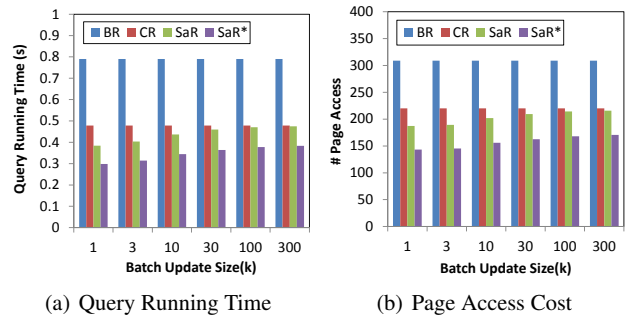
Fig. 17 The performance of the lazy update model on Gowalla.
