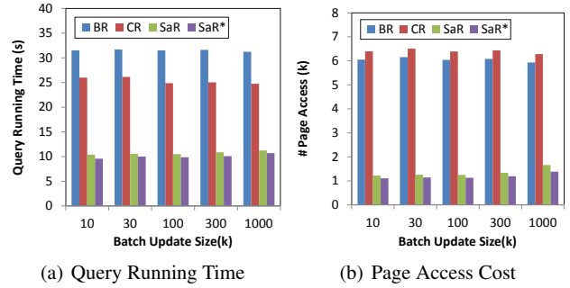
Fig. 18 The performance of the lazy update model on Twitter-2010.
