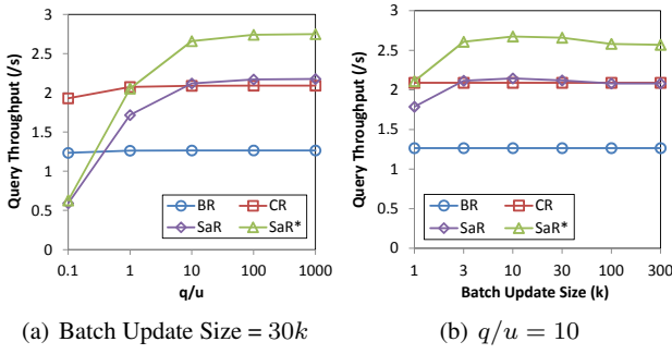
Fig. 19 The query throughput of the methods on Gowalla.
