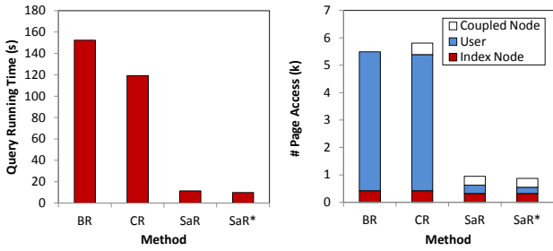
(e) GSGQ_{kNN} ( k=20, c=2 ) (f) GSGQ_{kNN} ( k=20, c=2 )
