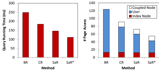
(a) GSGQ_{range} ( r=0.002, c=4 ) (b) GSGQ_{range} ( r=0.002, c=4 )
