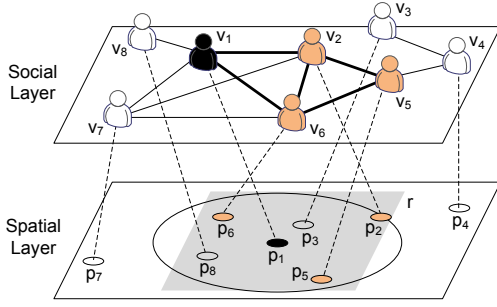
Fig. 1 An example of \text{GSGQ} \langle v_1, 3NN, 2 \rangle . Lines between the users represent acquaintance relations and the points on the spatial layer denote the positions of the users.
